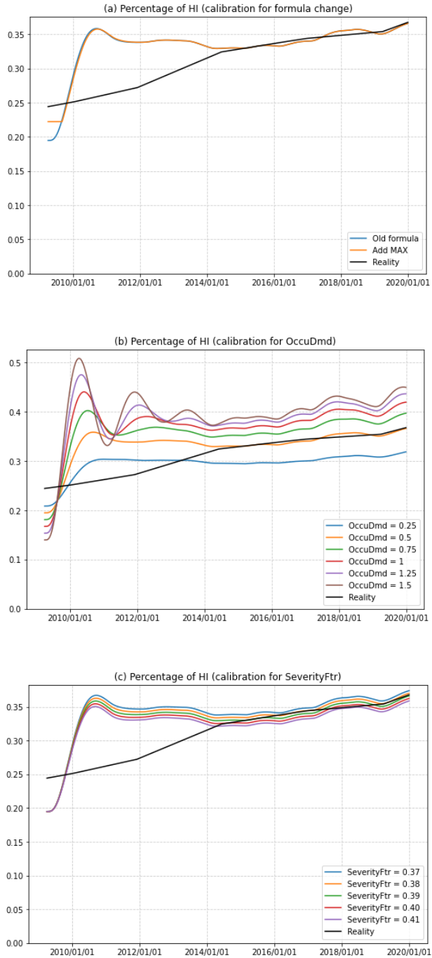
Figure S1: Graphical result for simulated percentage of health insurance vs. reality when calibrating for (a) adding MAX to formula (7); (b) OccuDmd; (c) SeverityFtr.
