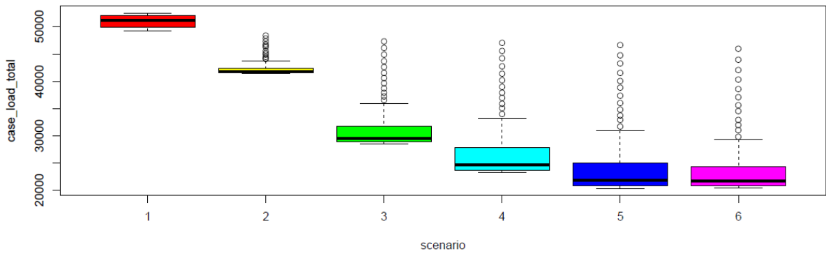
Figure A25: Impact of effectiveness_constant on case_load_total
